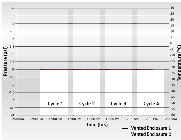
FIGURE 4: PRESSURE DIFFERENTIALS FOR VENTED ENCLOSURES
